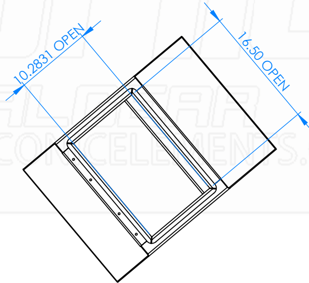
VIEW C SCALE 1 : 13
